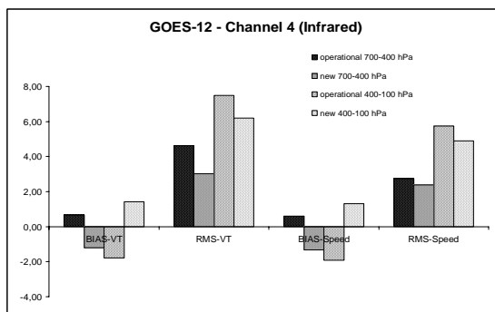
Figure 7 – Evaluation of the infrared CDW using the new spatial consistency test for, January 2006.
