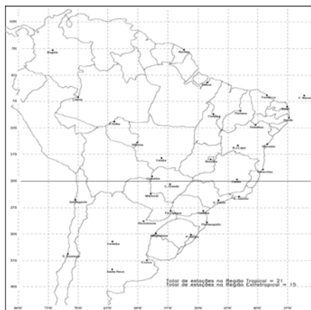
Figure 5 – Shows the radiosonde station available for evaluation of CDW.
