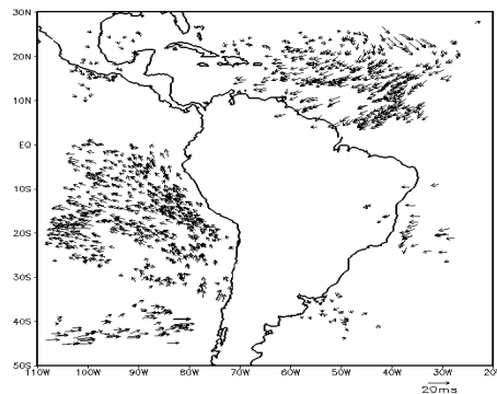
Figure 4: Low level winds computed using GOES-12 3.9 \mu\text{m} channel, for the day 24 March 2005 at 01:22Z
