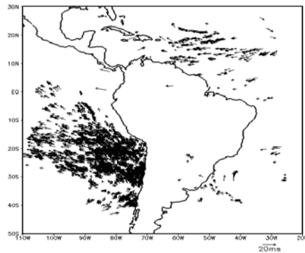
Figure 3: Low level winds computed using GOES-12 visible channel, for the day 24 March 2005 at 1522 Z
