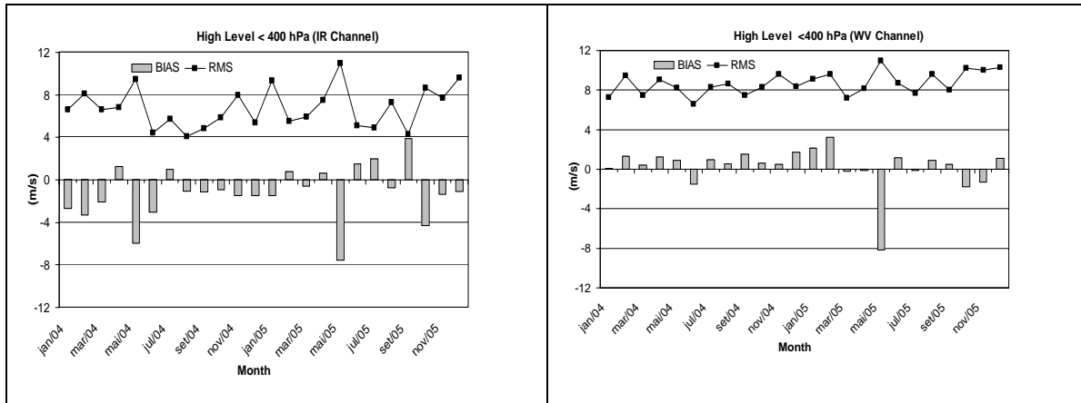
Figure 6 – RMS and BIAS for High level winds computed for GOES-12 infrared and water vapor channel.
