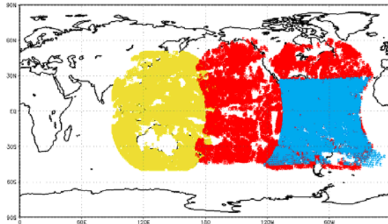
Figure 8 – CDW data assimilated in GPSAS on October, 10th 2005: a) from JMA (Yellow), b) from NOAA (red), c) from CPTC-DSA (blue) (overwriting part of NOAA data)
