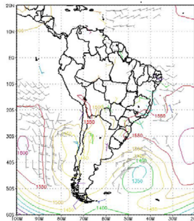
Figure 9 – GPSAS Analysis of Geopotential Height at 850 hPa (isolines) and observed winds assimilated by GPSAS from radiosondes station (barb if colors) and CDW (gray barb)
