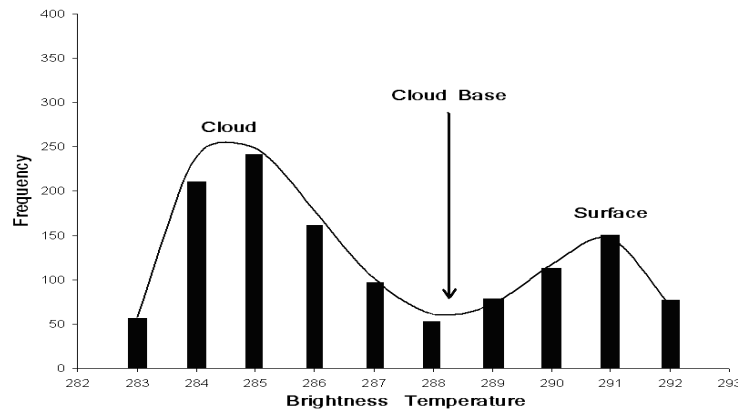
Figure 2: Schematic view of the histogram computed for height assigned.
