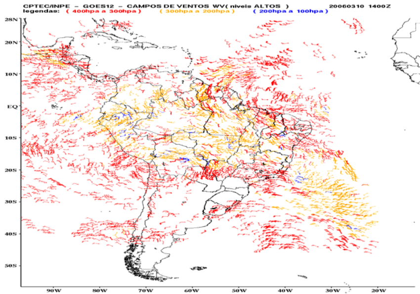
Figure 1- Example of winds computed operationally at CPTEC. CDW computed for high levels using GOES-12 water vapor channel.
