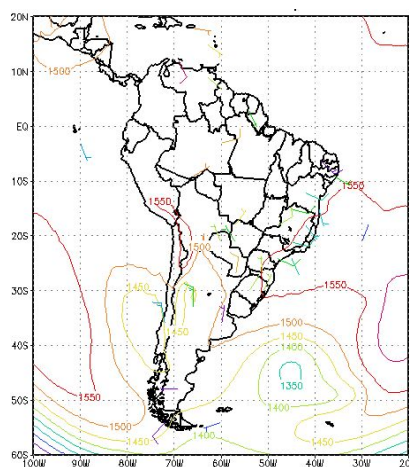
Figure 10 – GPSAS analyse of Geopotential Height at 850 hPa (isolines) and radiosondes winds assimilated by GPSAS
